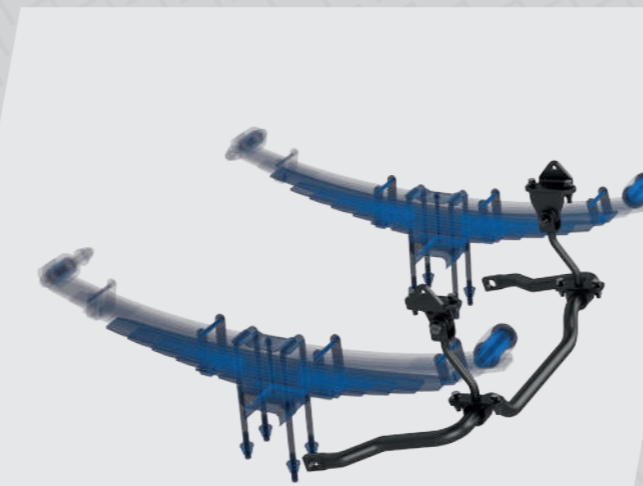
Anti-roll Bar
